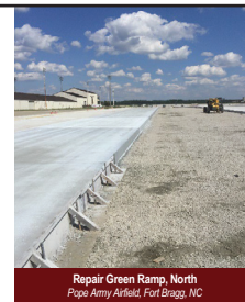
Repair Green Ramp, North Pope Army Airfield, Fort Bragg, NC
